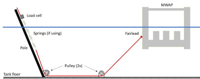
Fig. 8. Schematic of mooring implementation in the tank with waterline in blue.
