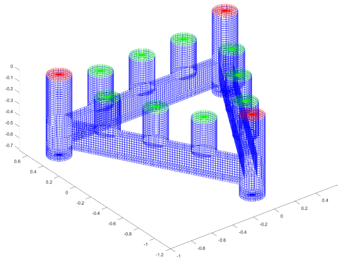
Fig. 9. Boundary element panels for WAMIT analysis of 9 WEC platform case, where generalized modes are applied to absorber surfaces shown in green.
