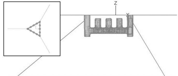
Fig. 6. Image from ORCAFLEX modelling showing 'compliant' mooring layout analysed. Note additional compliance in this case is provided by springs attached at line termination point (see Fig. 8). Inset: plan view.
